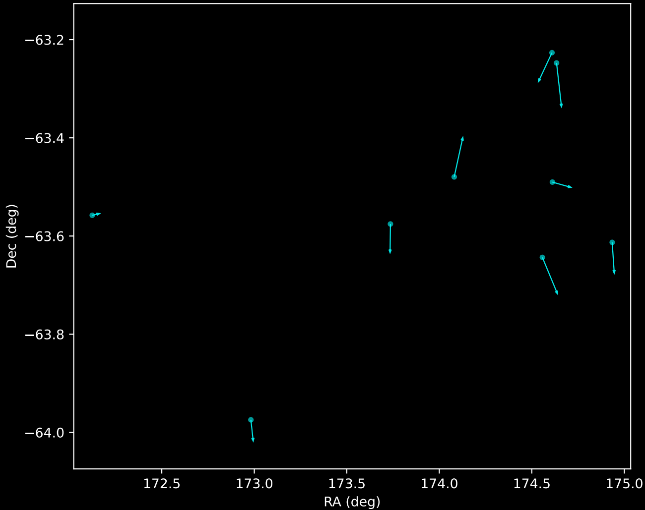
APOGEE DR17 Noise Stream Proper Motion Vectors (n=9)
