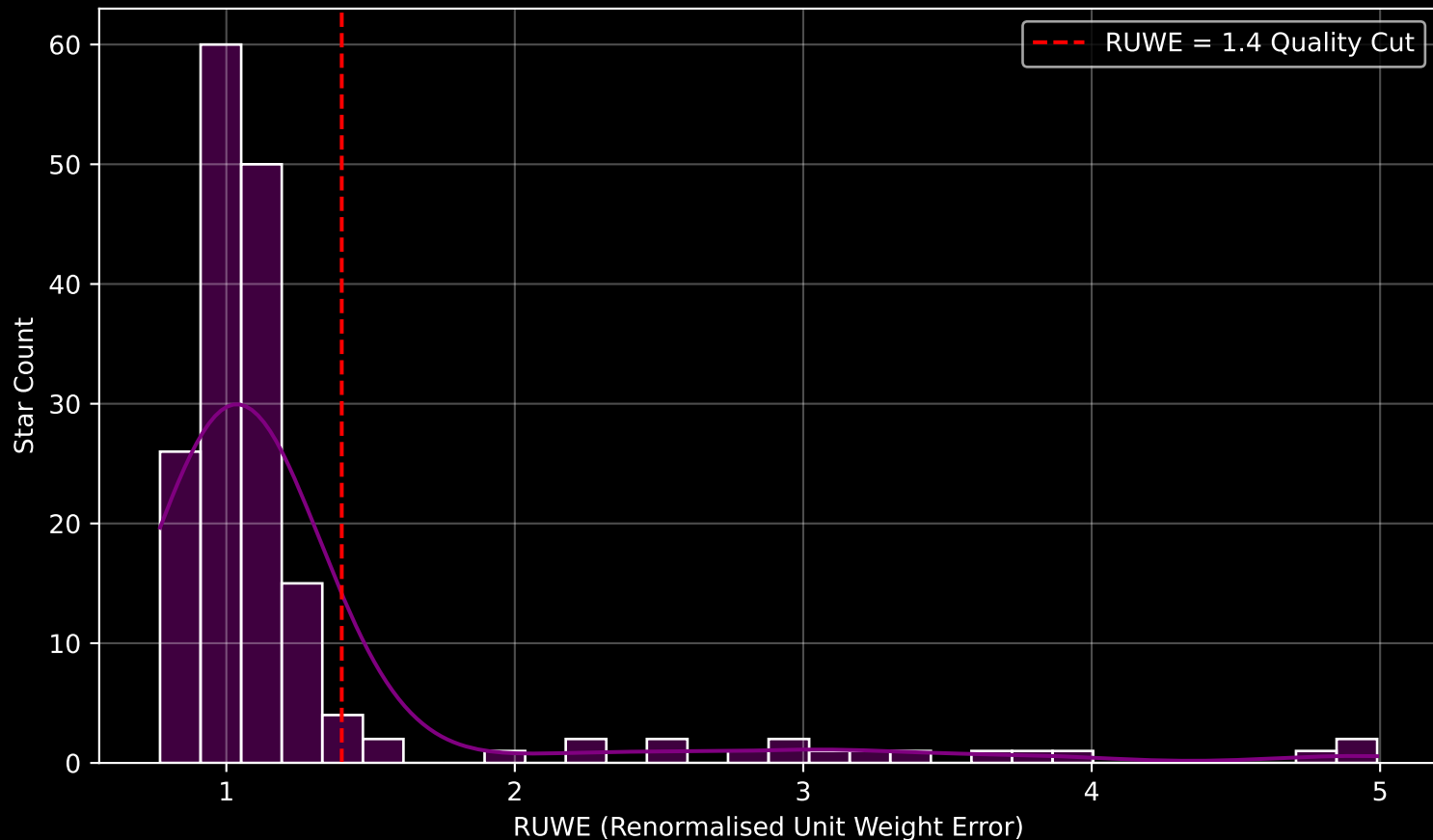
GAPOGEE DR17 Field [273-37-O_TESS] RUWE Distribution (n= 174)
