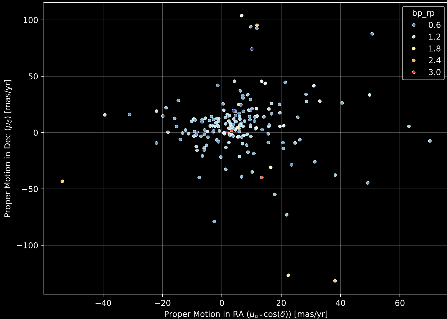
APOGEE DR17 Field: [273-37-O_TESS] Proper Motion Diagram (n= 187)
