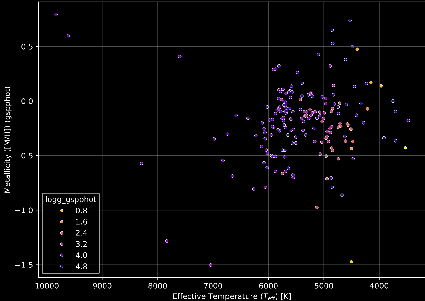
APOGEE DR17 Field: [273-37-O_TESS] Stellar Population Parameters (n= 187)
