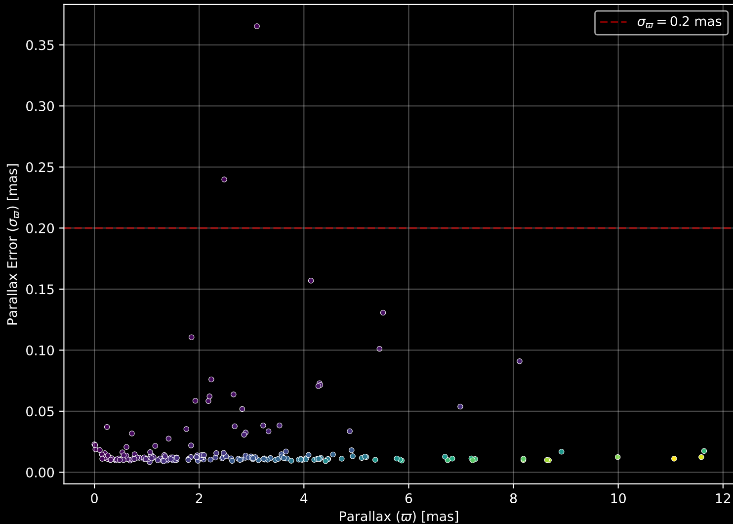
APOGEE DR17 Field: [273-37-O_TESS] Parallax Quality (n= 187)
