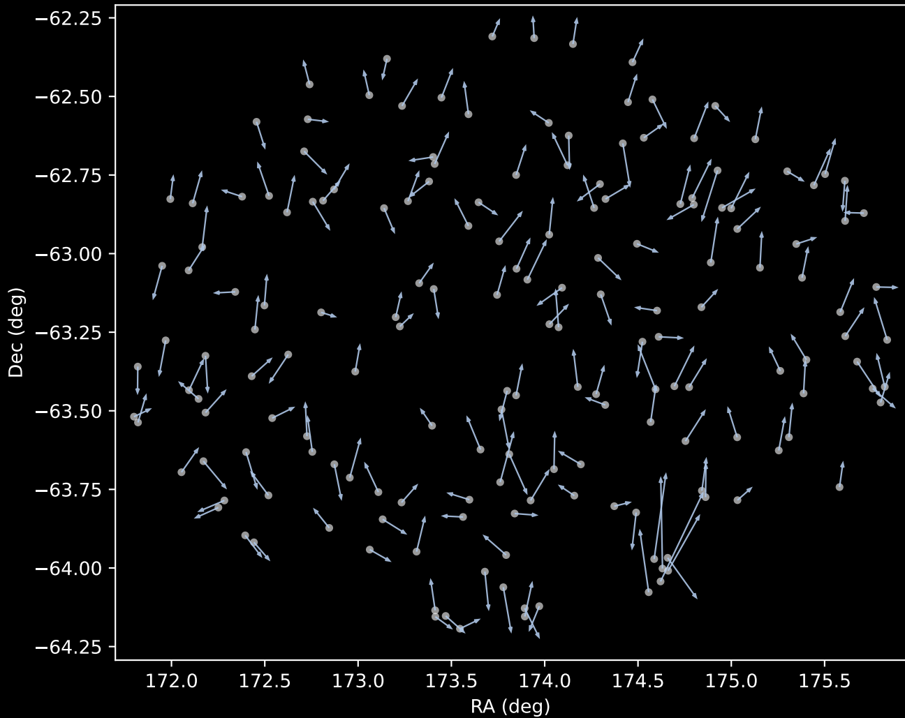
APOGEE DR17 Cluster 1 Proper Motion Vectors (n=173)
