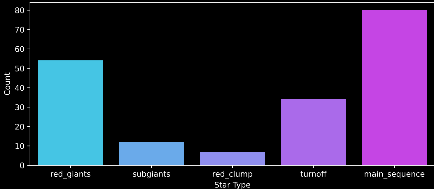
APOGEE DR17 Field: [273-37-O_TESS] Count plot of Star Type
