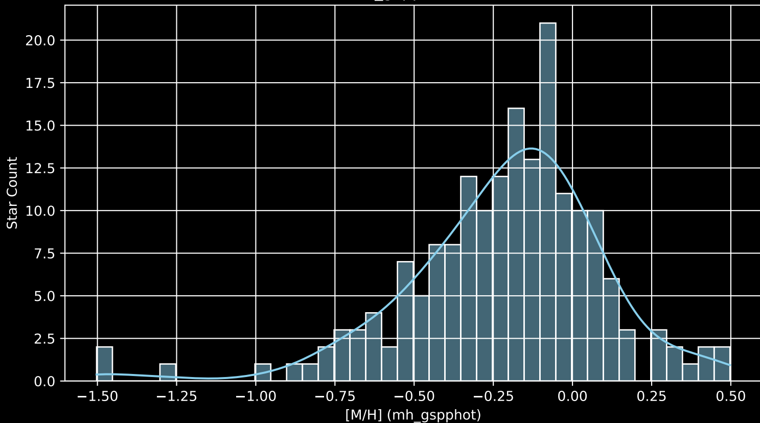
APOGEE DR17 Field: [273-37-O_TESS [M/H] (mh_gspphot) (n= 182)
