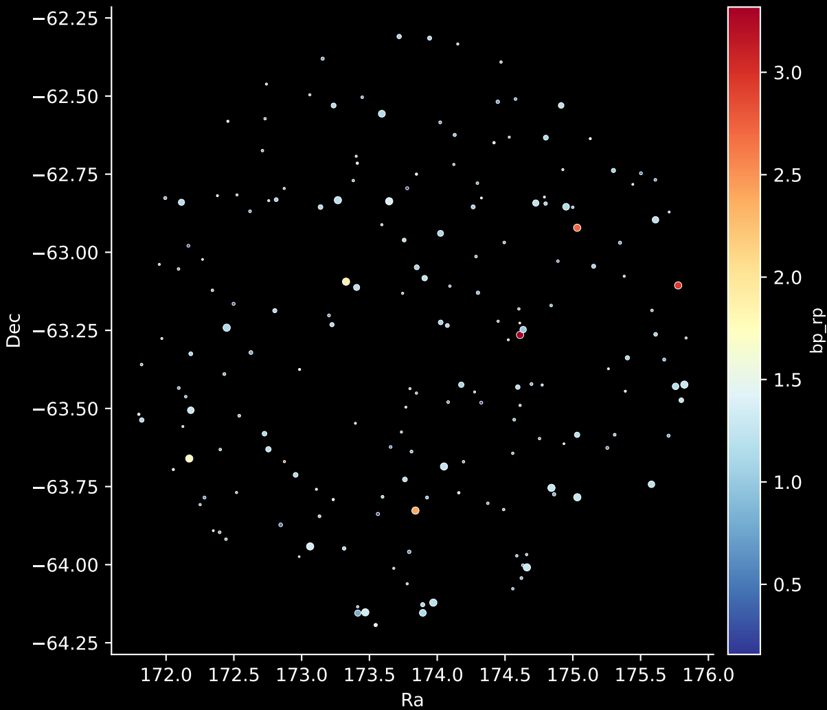
APOGEE DR17 Field: [273-37-O_TESS] Stars: 187
